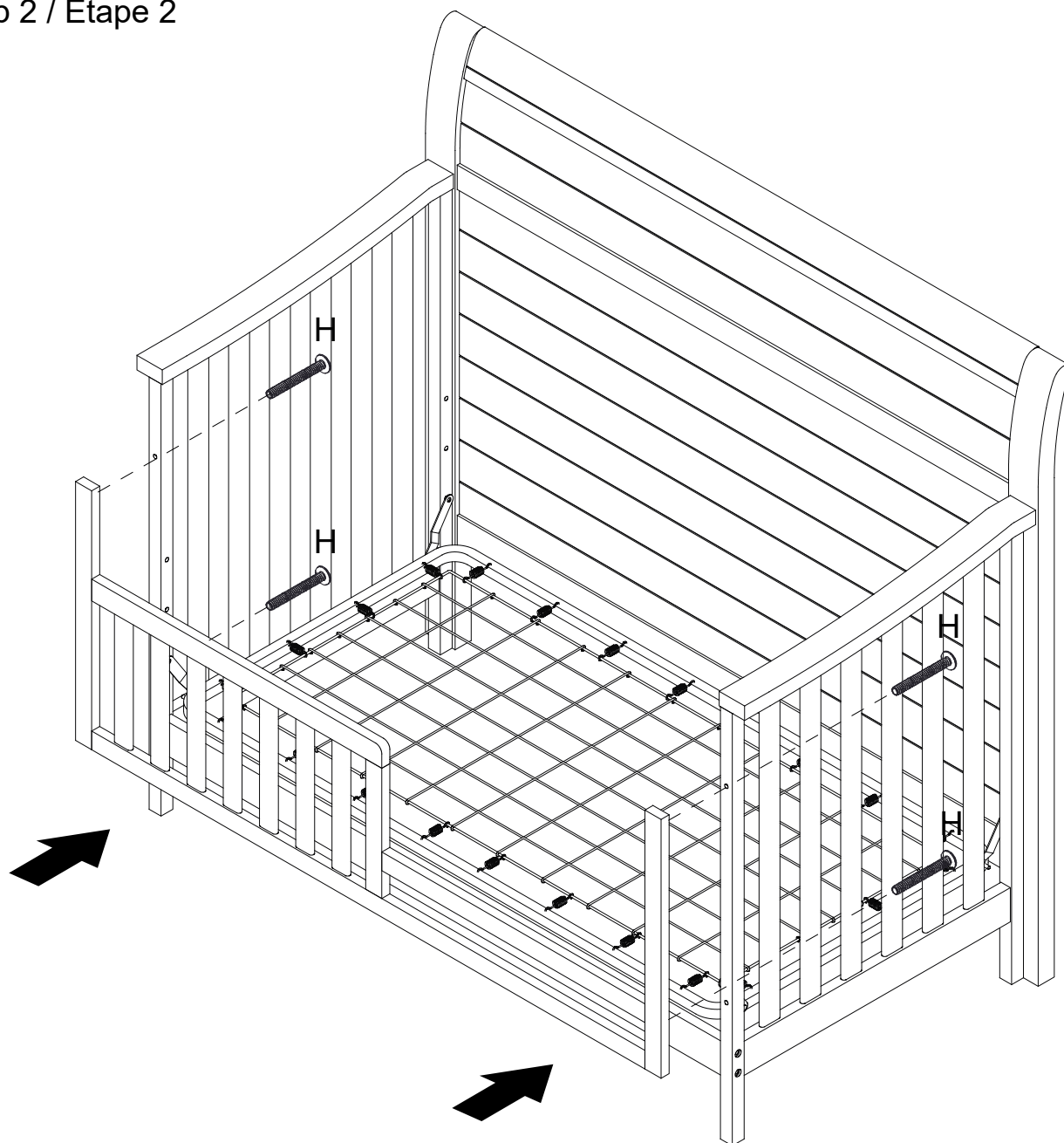
(H) M6 x 35mm Allen Bolt / Boulon Allen (x 4)
